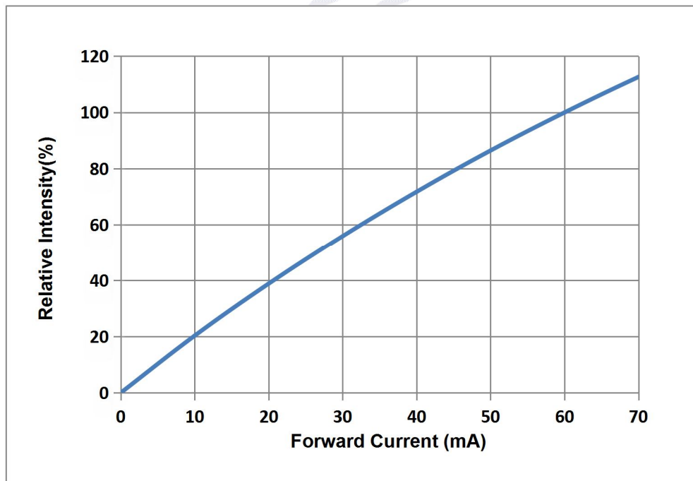
Fig 1-8 Forward Current Vs. Relative Intensity 正向电流与相对光强特性
