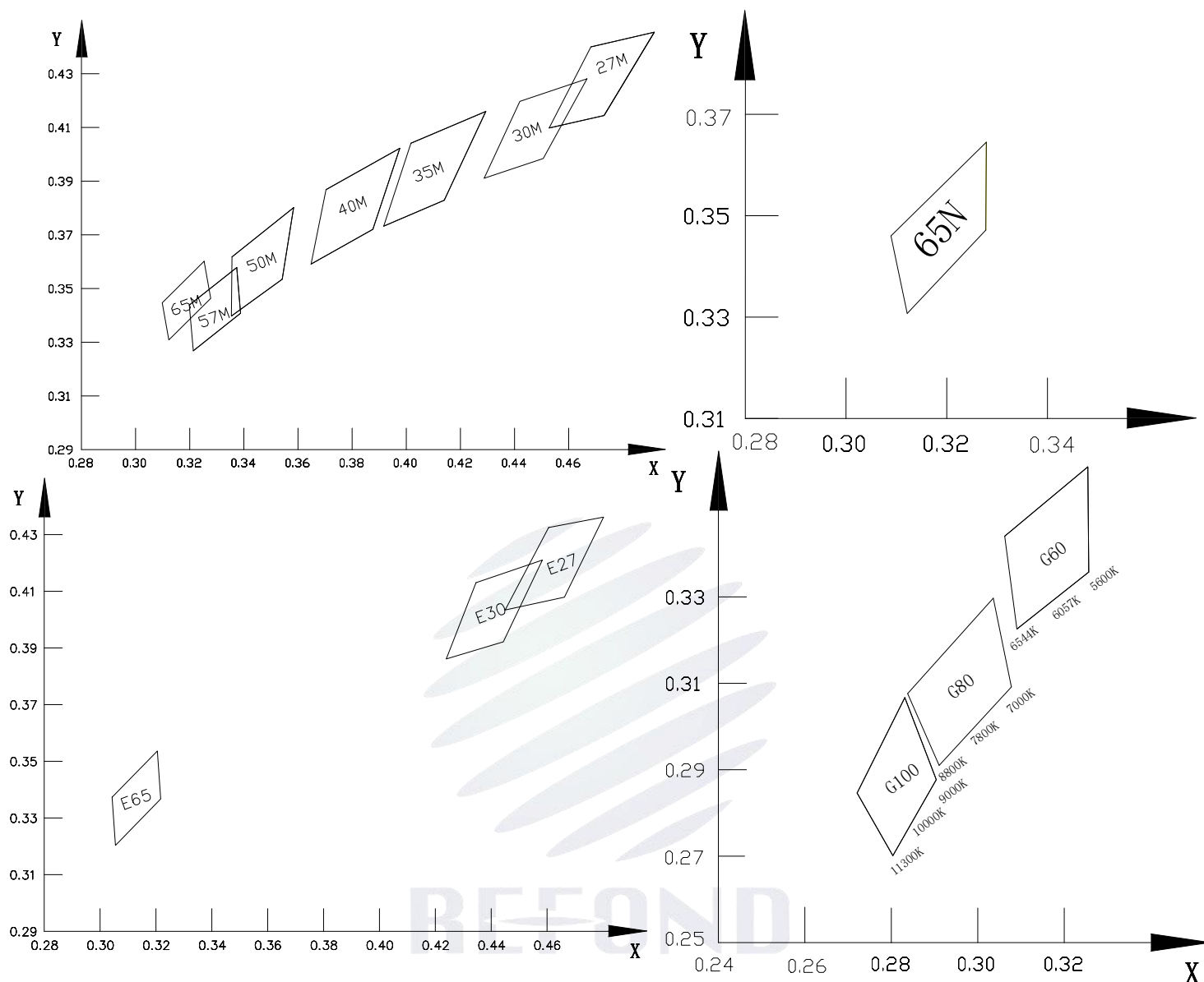
Fig 1-6 The C.I.E Chromaticity Diagram CIE色度图
