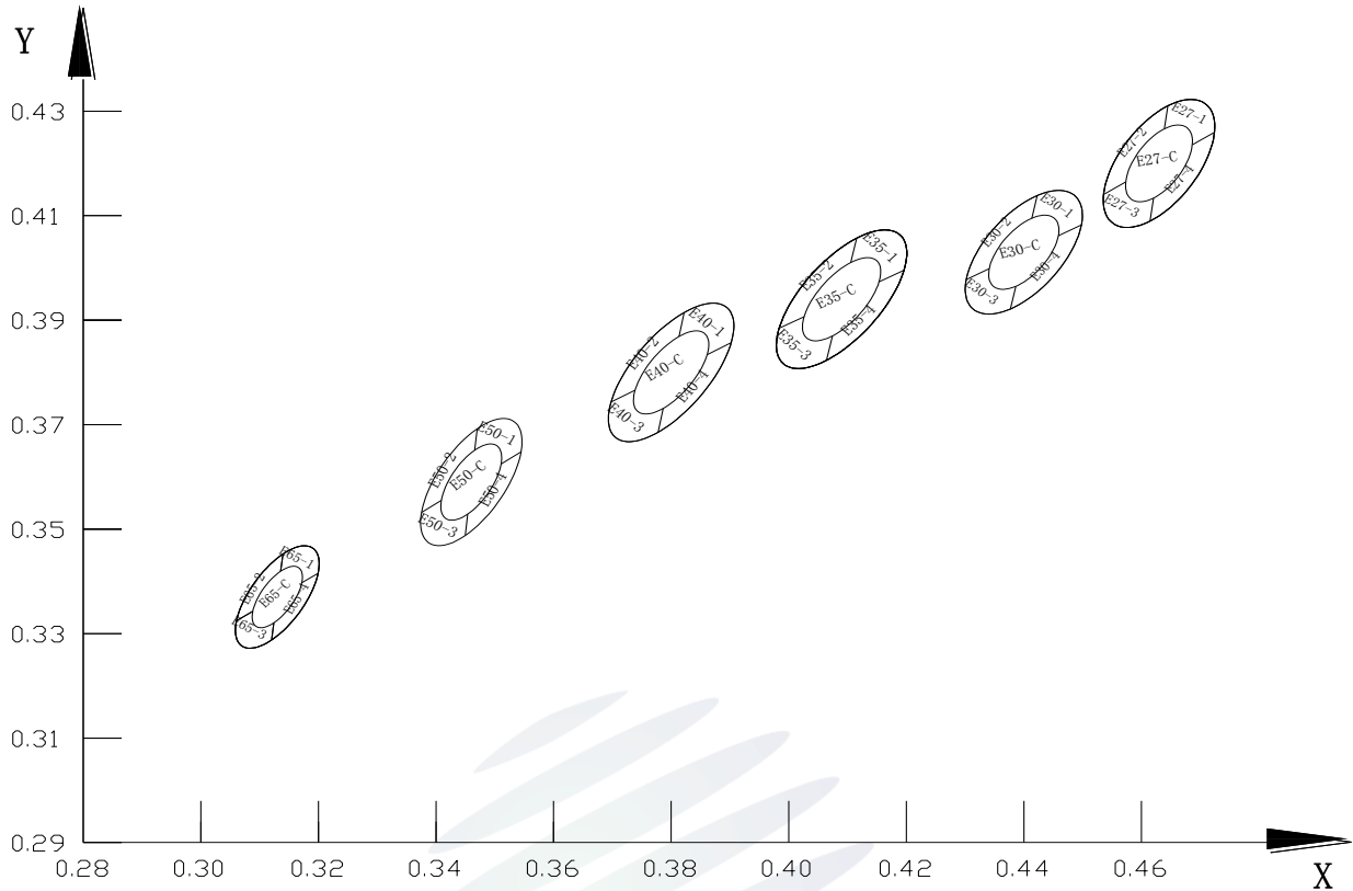
Fig 1-6 The C.I.E Chromaticity Diagram CIE色度
